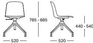
TRESTLE BASE
