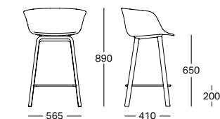
WOOD FRAME H650
