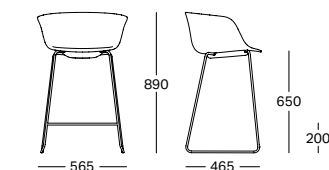
SLED FRAME H650
