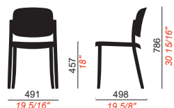
MONOSHELL 4 LEGS
