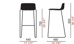
4 LEGS FRAME
