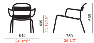
4 LEGS FRAME
