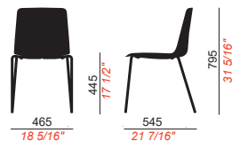
4 LEGS FRAME
