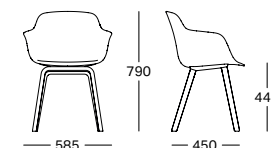
4 LEGS FRAME
