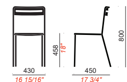
4 LEGS FRAME
