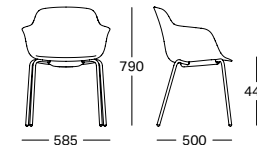
4 LEGS FRAME
