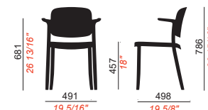
MONOSHELL 4 LEGS
