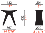
2 LEGS STOOL
