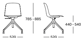
TRESTLE BASE
