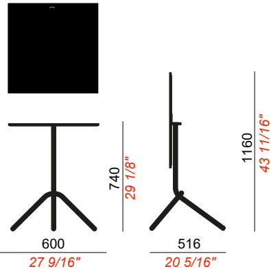
BASE 3 PIEDI, TOP DIAM. 600 3 FEET BASE, TOP DIAM. 600
