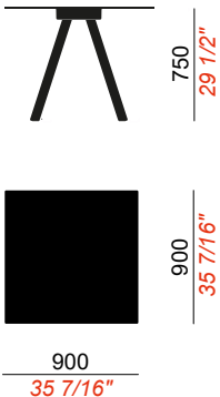
BASE 4 PIEDI, PIANO 900X900 4 FEET BASE, TOP 900X900
