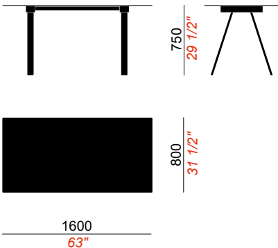
BASE 4 PIEDI, PIANO 1600X800 4 FEET BASE, TOP 1600X800
